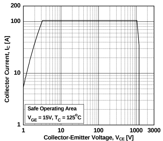
Figure 18. Turn off Swtting SOA Characteristics
