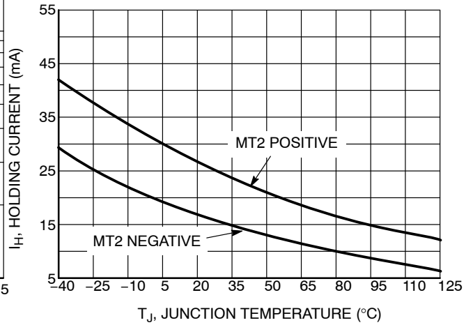
Figure 5. Hold Current Variation
