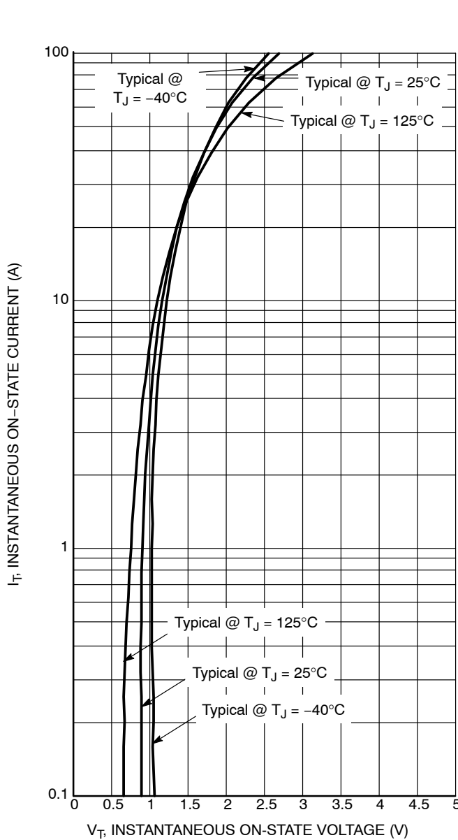
Figure 3. On-State Characteristics
