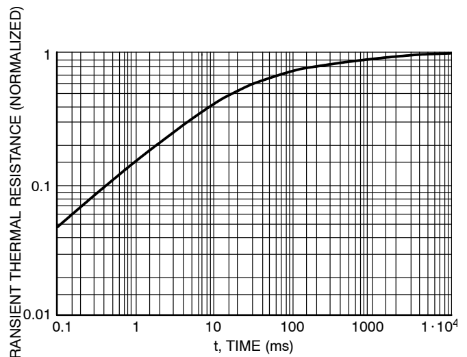
Figure 4. Thermal Response
