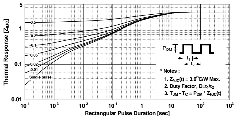
Figure 10. Transient Thermal Response Curve - FDPF10N60ZUT
