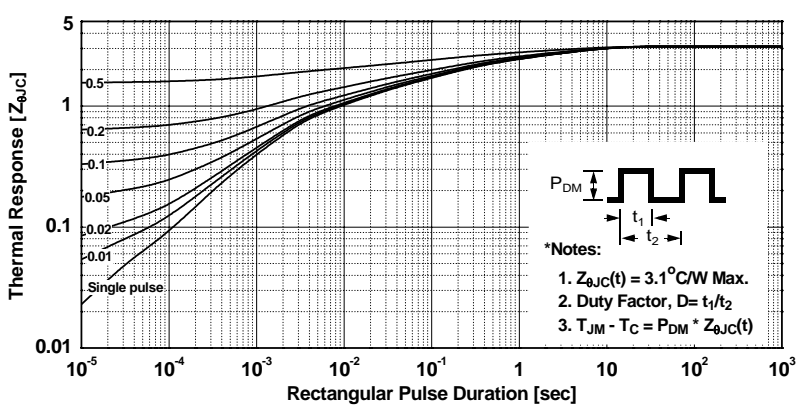
Figure 13. Transient Thermal Response Curve - FDPF8N50NZT
