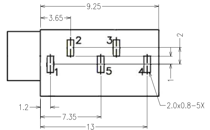
DIMENSIONS OF PC BOARD HOLES TOLERANCE ±0.1 (TOP VIEW)
