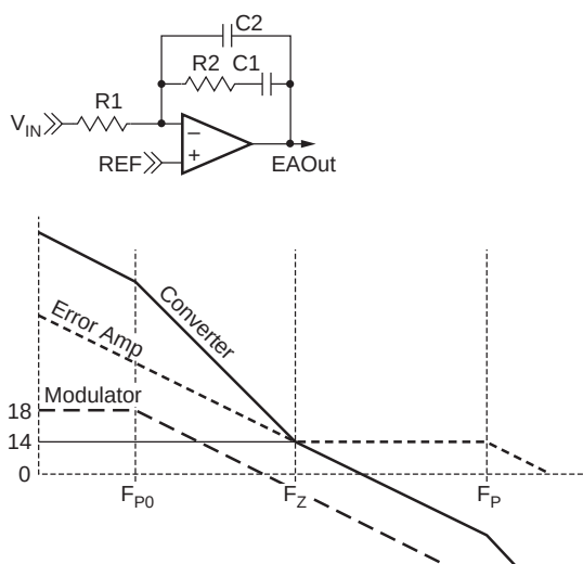
Figure 9. Compensation
