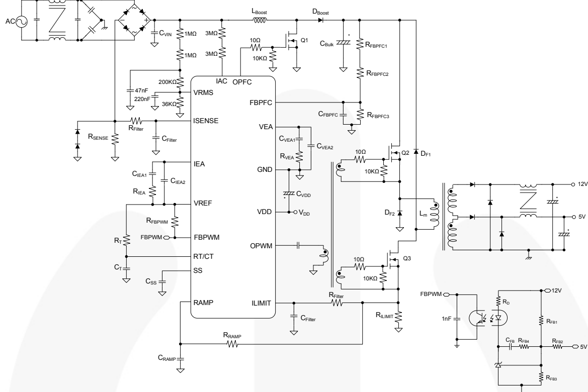
Figure 2. Current Mode
