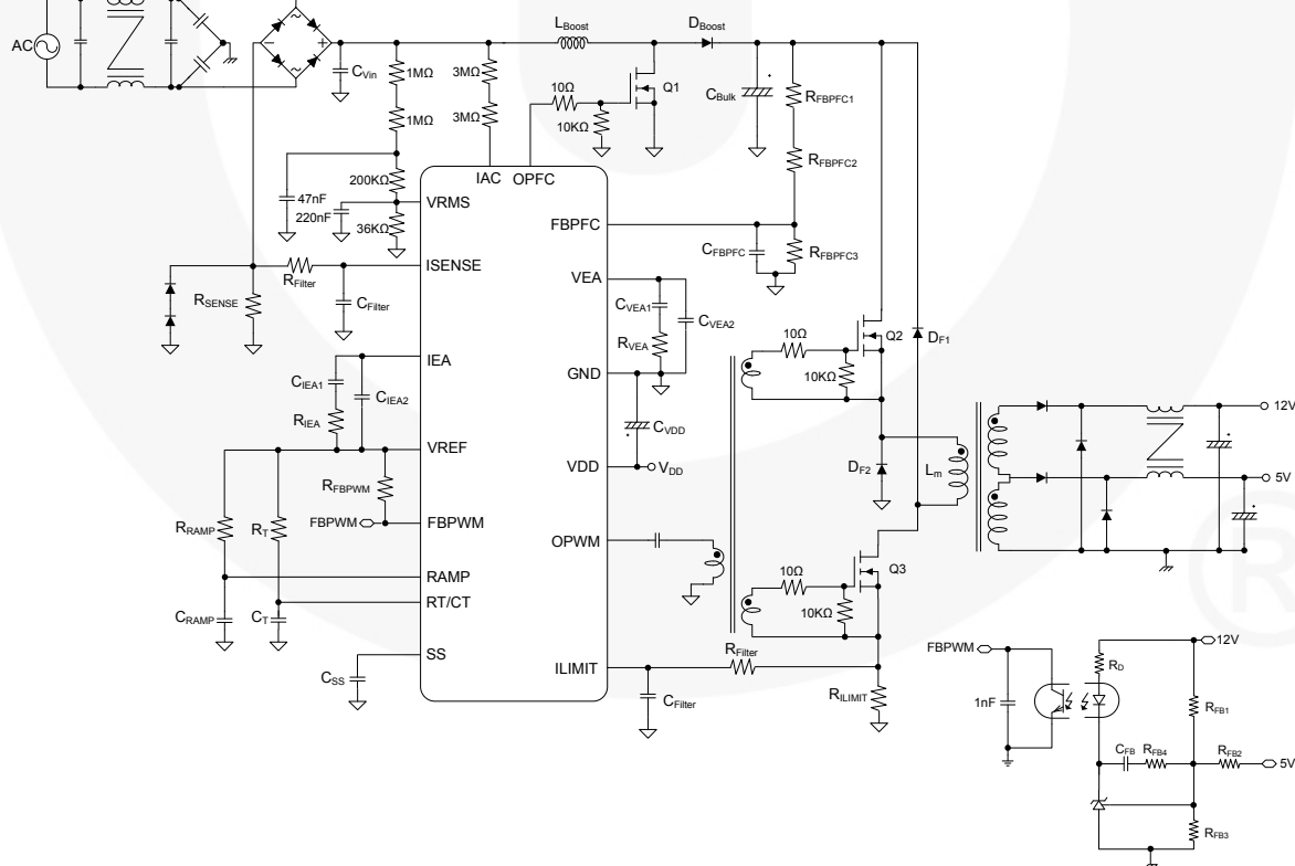
Figure 3. Voltage Mode
