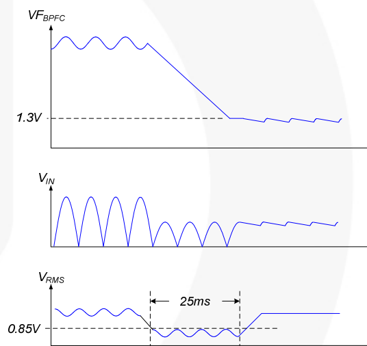
Figure 38. The Second condition of Sag Protection
