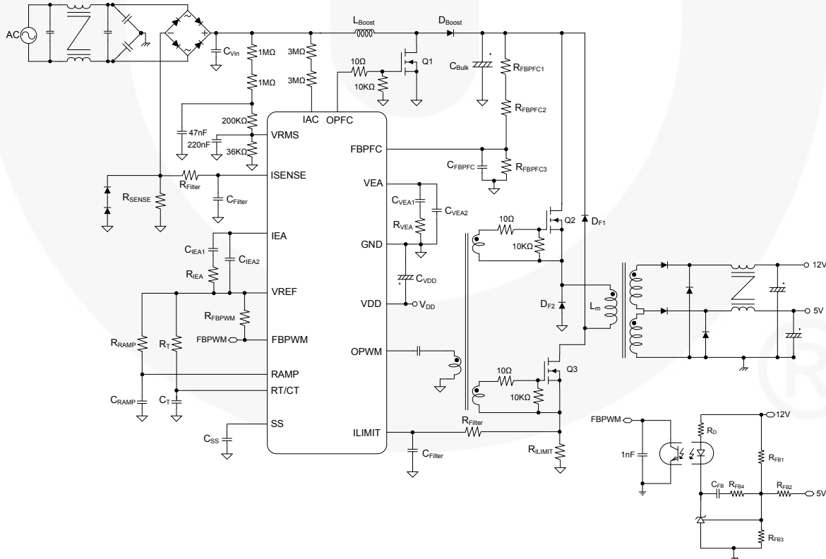
Figure 3. Voltage Mode
