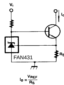
Figure 17. Constant-Current Sink
