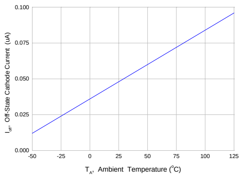
Figure 6. OFF-State Cathode Current vs. Ambient Temperature
