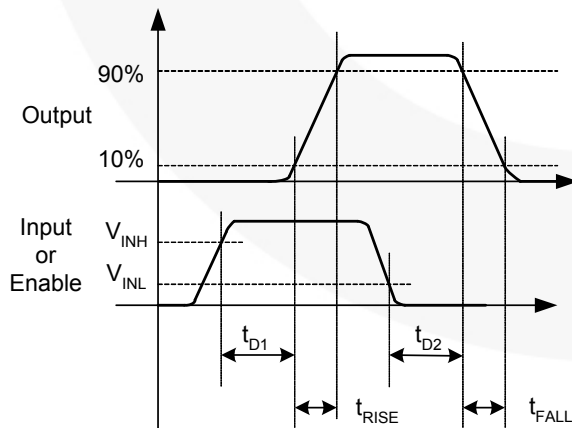
Figure 5. Non-Inverting
