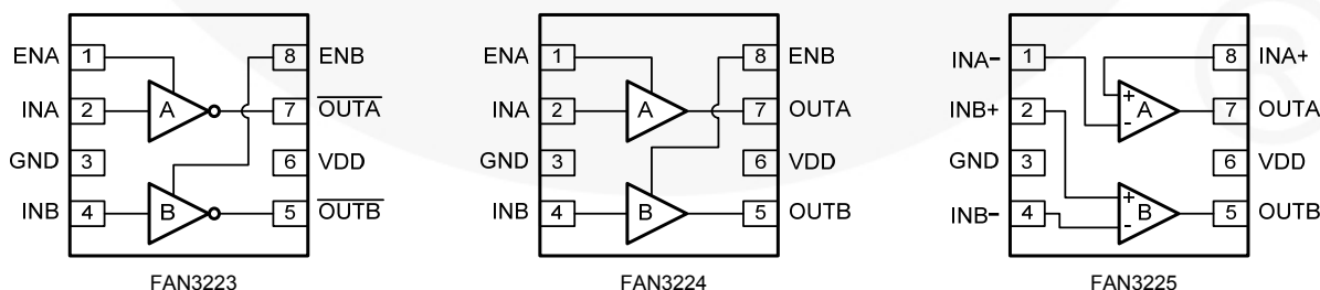
Figure 1. Pin Configurations
