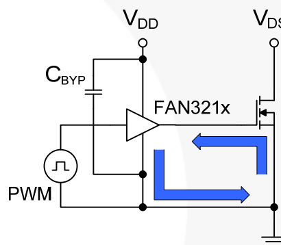
Figure 31. Current Path for MOSFET Turn-Off
