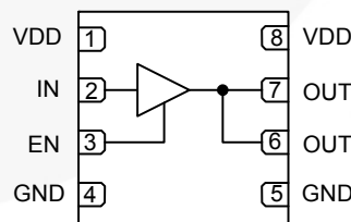
Figure 2. FAN3122 Pin Configuration
