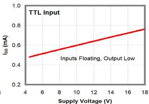
Figure 11. I_{DD} (Static) vs. Supply Voltage (12)
