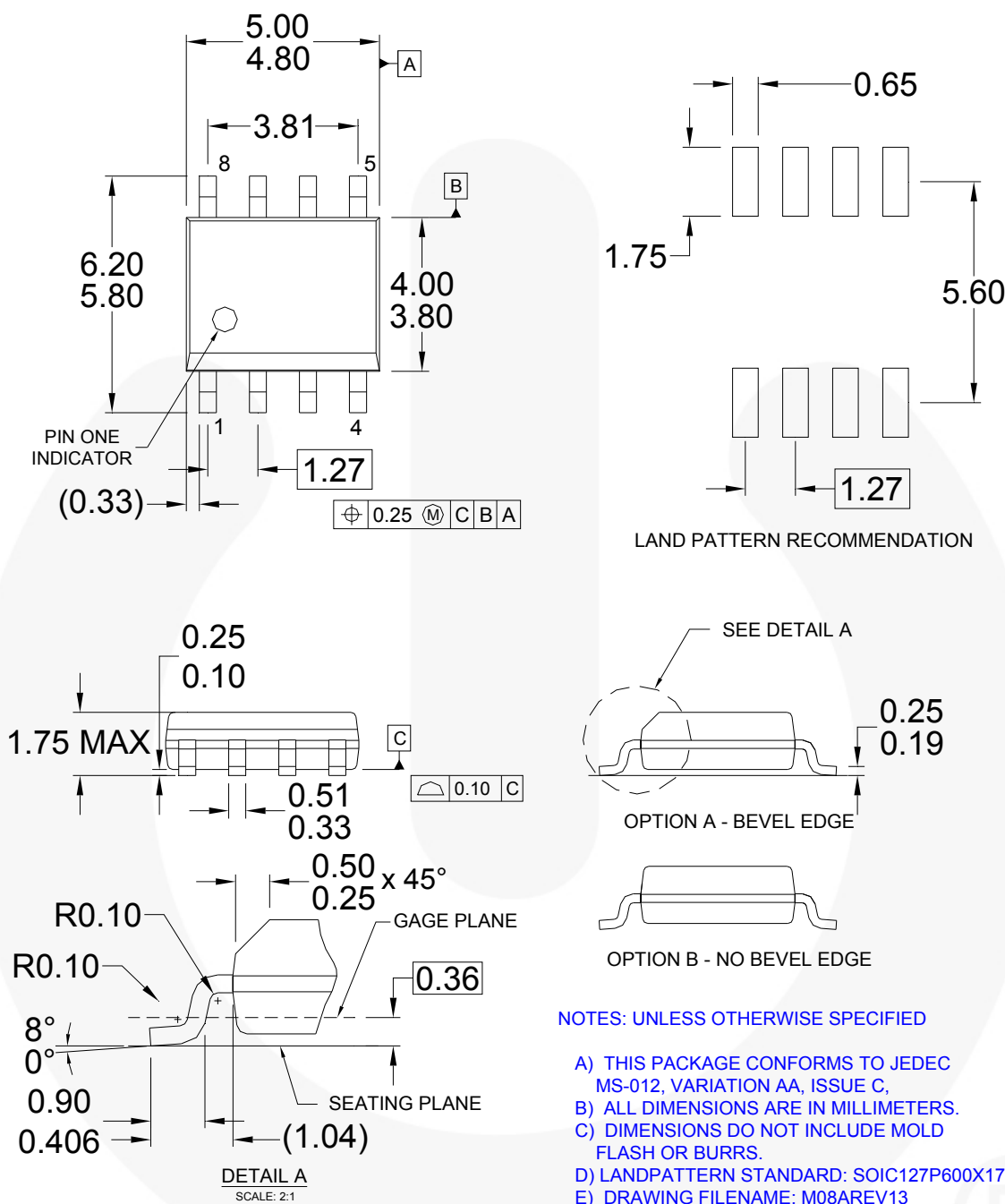
Figure 56. 8-Lead Small Outline Integrated Circuit (SOIC)
