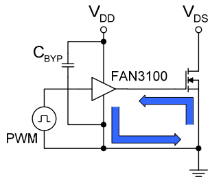
Figure 44. Current Path for MOSFET Turn-Off
