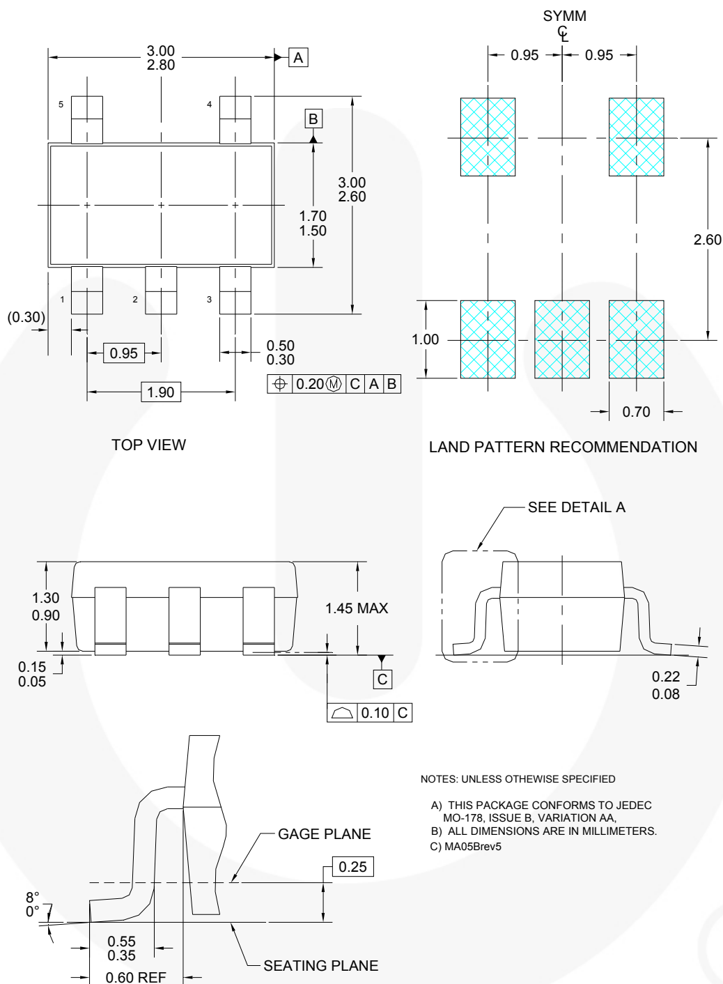
Figure 54. 5-Lead SOT-23
