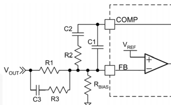
Figure 34. Compensation Network
