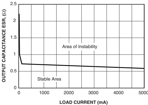
Figure 10. Stability Region V_{IN}/V_{OUT} = 5V/1.5V
