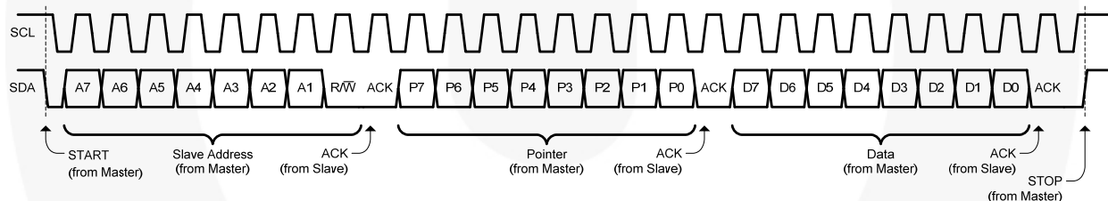
Figure 25. I²C Write
