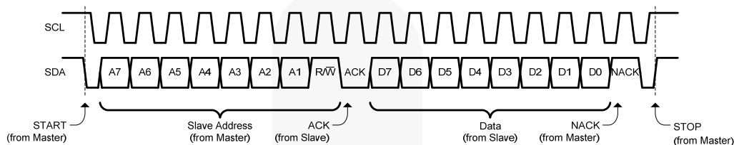
Figure 19. I²C Read
