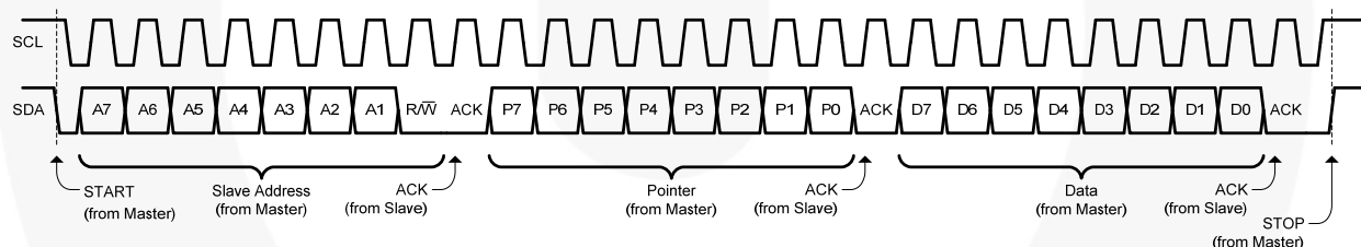
Figure 21. I²C Write
