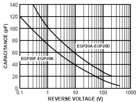
Junction Capacitance
