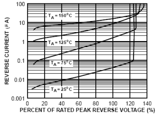
Reverse Characteristics
