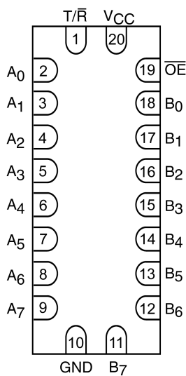
Pin Assignment for DQFN
