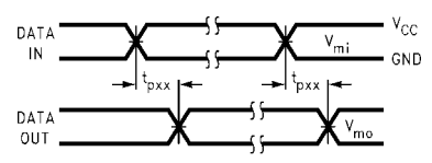
FIGURE 8. Waveform for Inverting and Non-Inverting Functions
