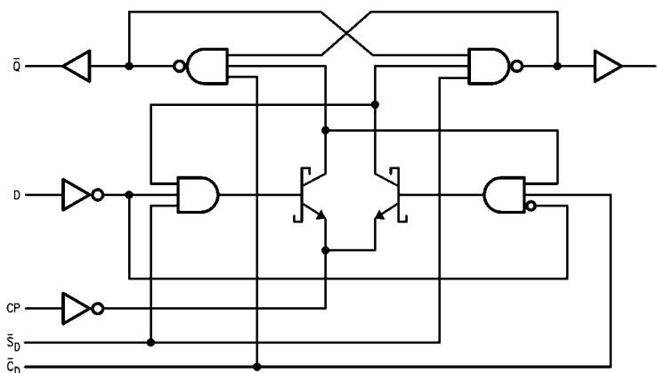
Logic Diagram
