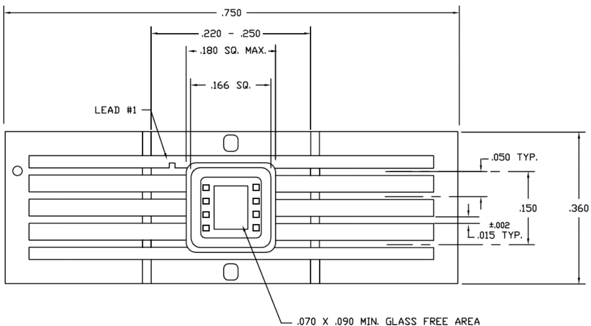
Figure 10. Package Drawing 8-lead CSOIC
