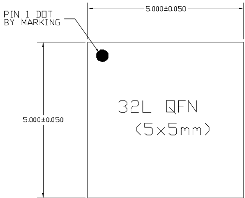
Figure 24. Package Drawing
