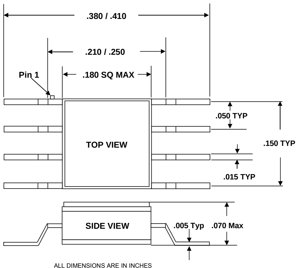
Figure 14. Package Drawing
