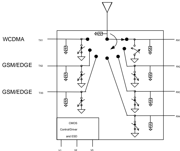
Figure 1. Functional Diagram
