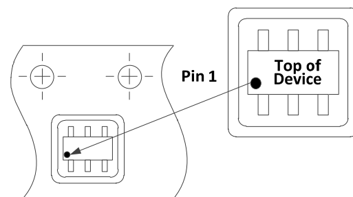
Device Orientation in Tape
