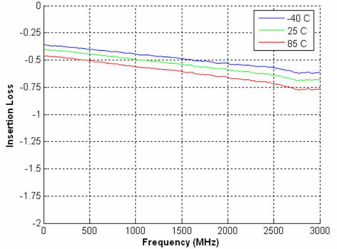
Figure 7. Insertion Loss: RFC-RF1 @ 3 V
