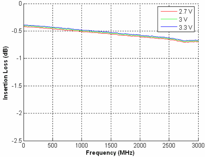
Figure 6. Insertion Loss: RFC-RF1 @ 25 °C
