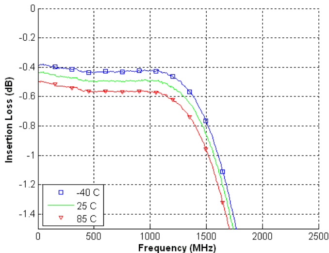
Figure 12. Rx Insertion Loss Attenuated, V_{DD}=3.3V
