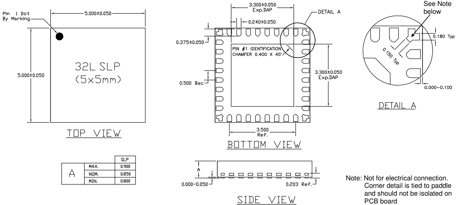
Figure 14. Package Drawing
