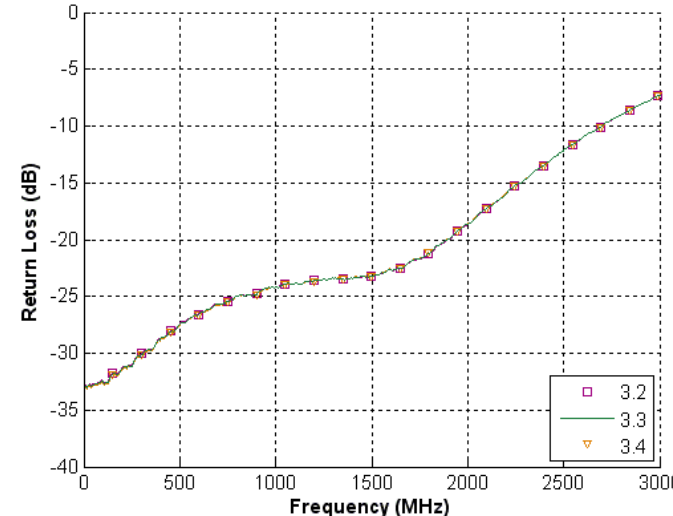
Figure 11. RF Return Loss, +25 °C
