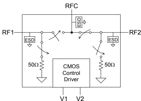
Figure 1. Functional Diagram
