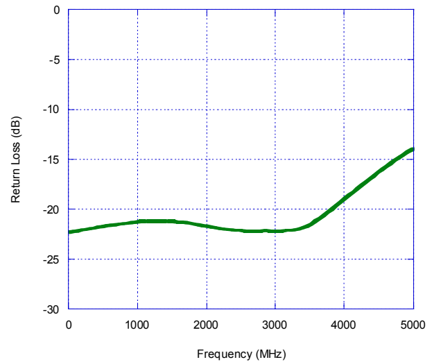
Figure 10. RF2 Return Loss (CTRL = Low)
