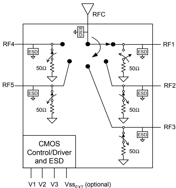
Figure 1. Functional Diagram
