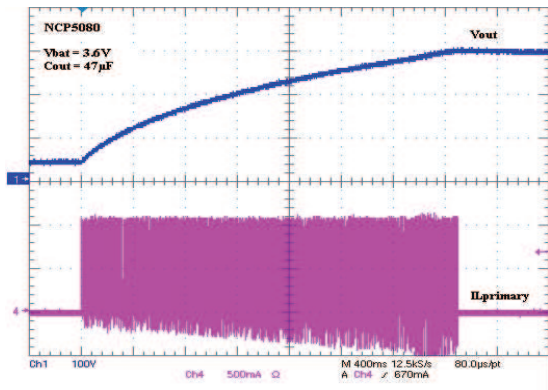
Figure 8. Output Capacitor Recharge Cycle
