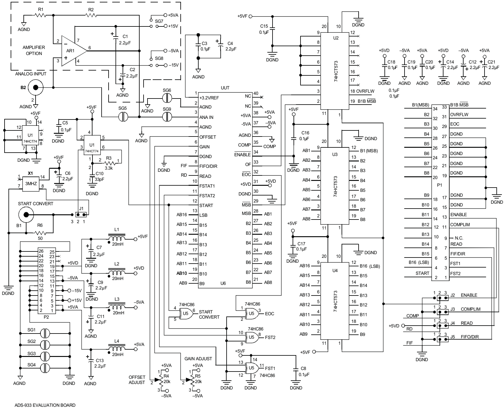
Figure 4. ADS-933 Evaluation Board Schematic
