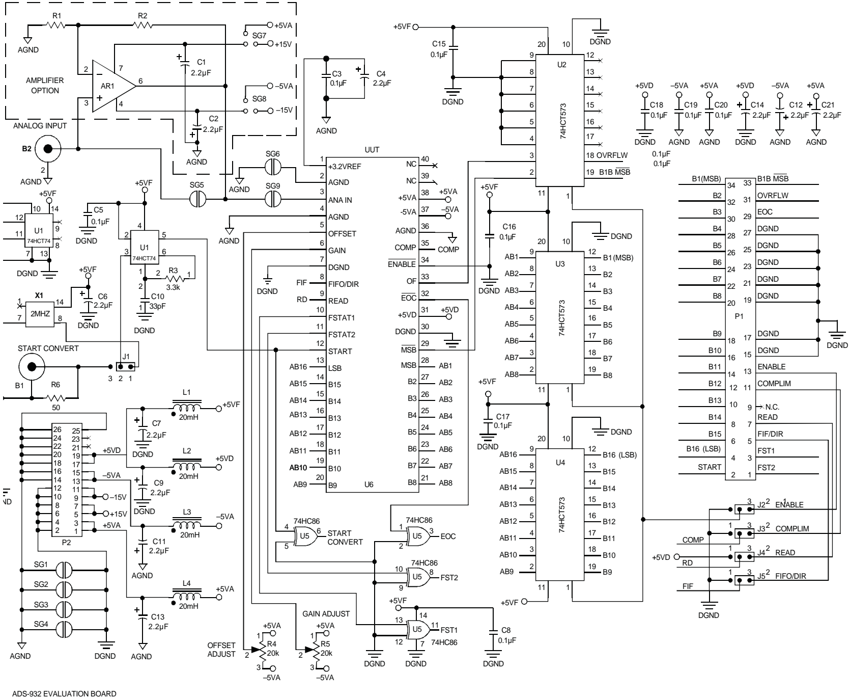
Figure 5. ADS-932 Evaluation Board Schematic
