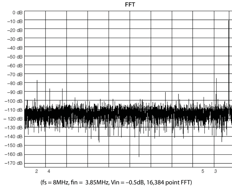
Figure 5. FFT Analysis of ADS-947
