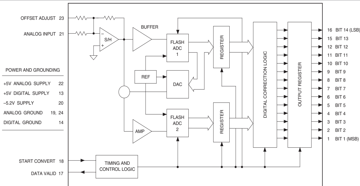
Figure 1. ADS-947 Functional Block Diagram
