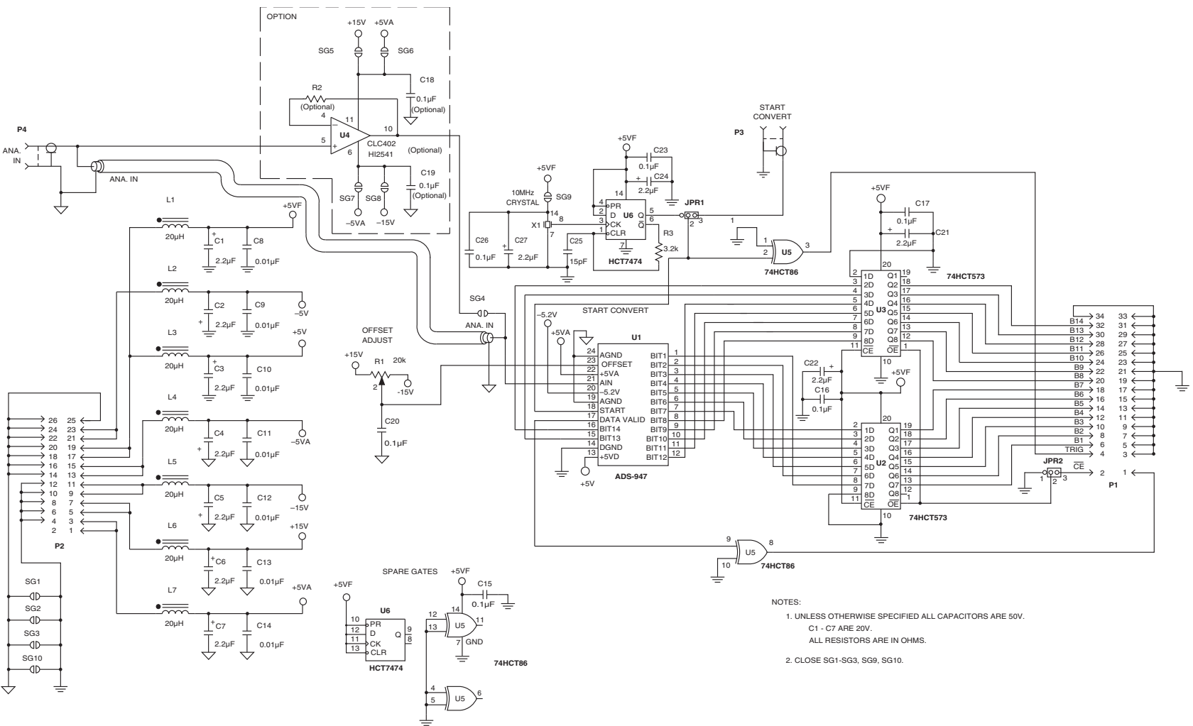
Figure 7. ADS-947 Evaluation Board Schematic (ADS-B947)
