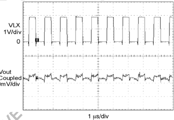
Figure 19. Heavy-Load PWM Switching Waveform ( V_{in} = 3.6\text{ V} , V_{out} = 1.5\text{ V} , I_{out} = 300\text{ mA} )
