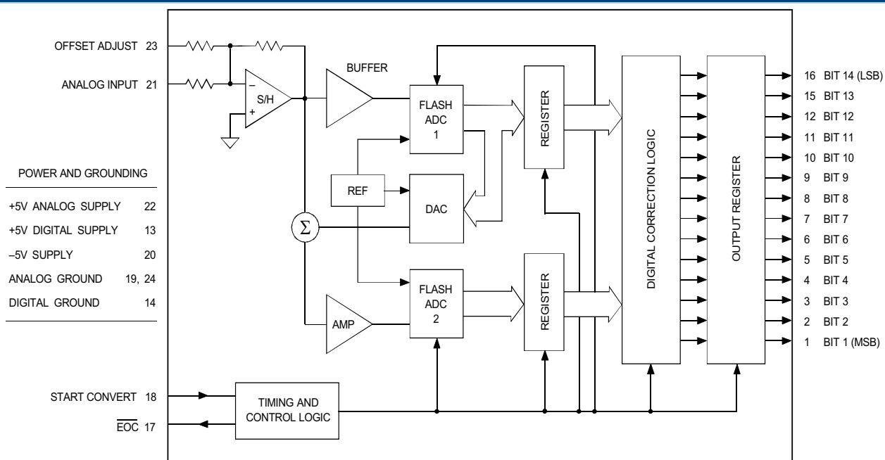
Figure 1. ADS-946 Functional Block Diagram
