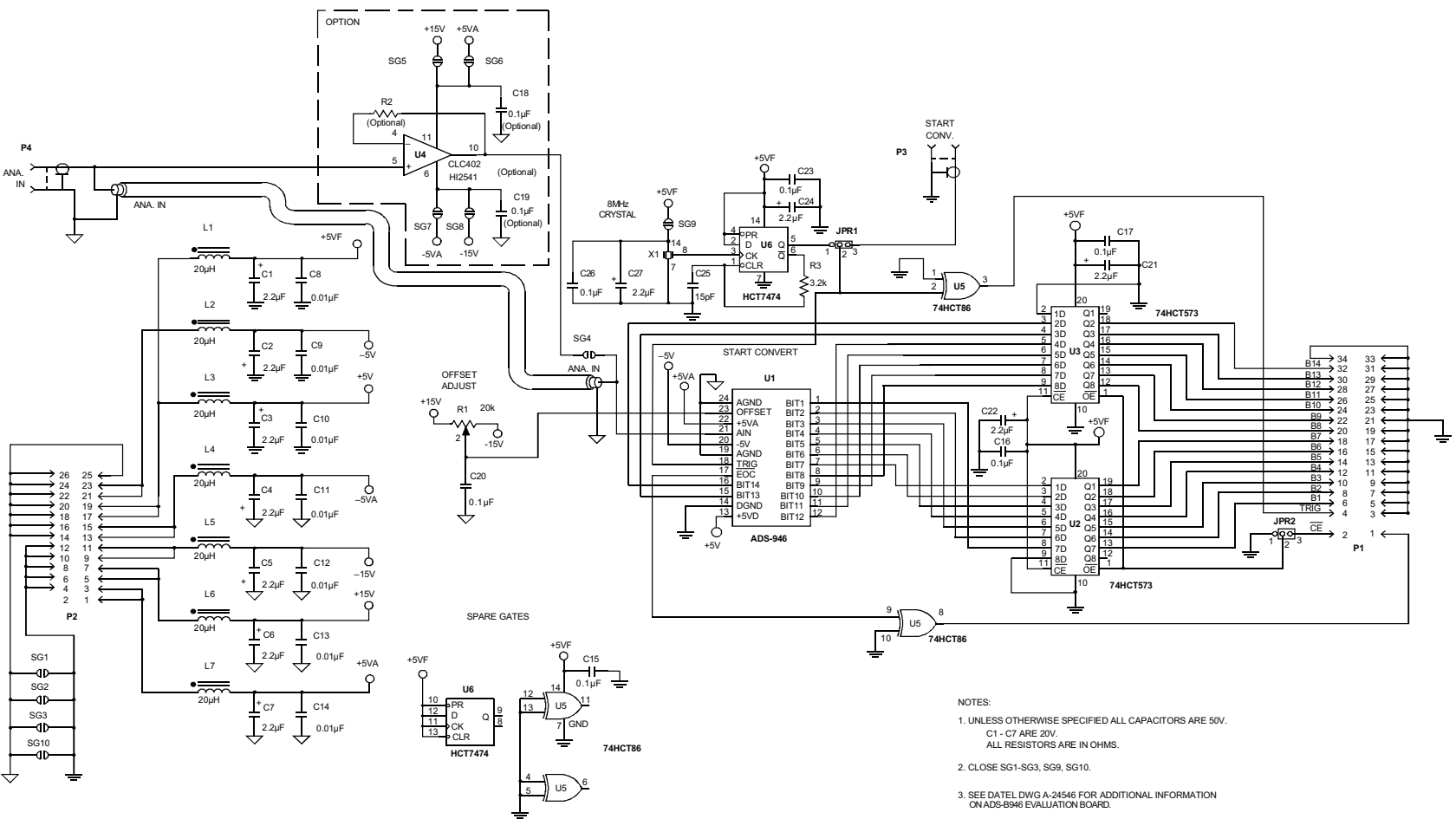
Figure 7. ADS-946 Evaluation Board Schematic (ADS-B946)
