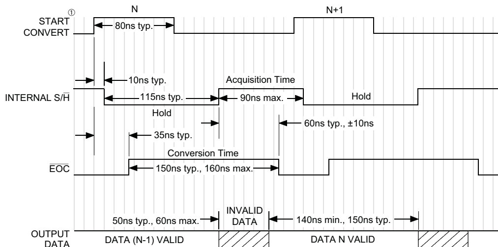
Figure 3. ADS-944 Timing Diagram
