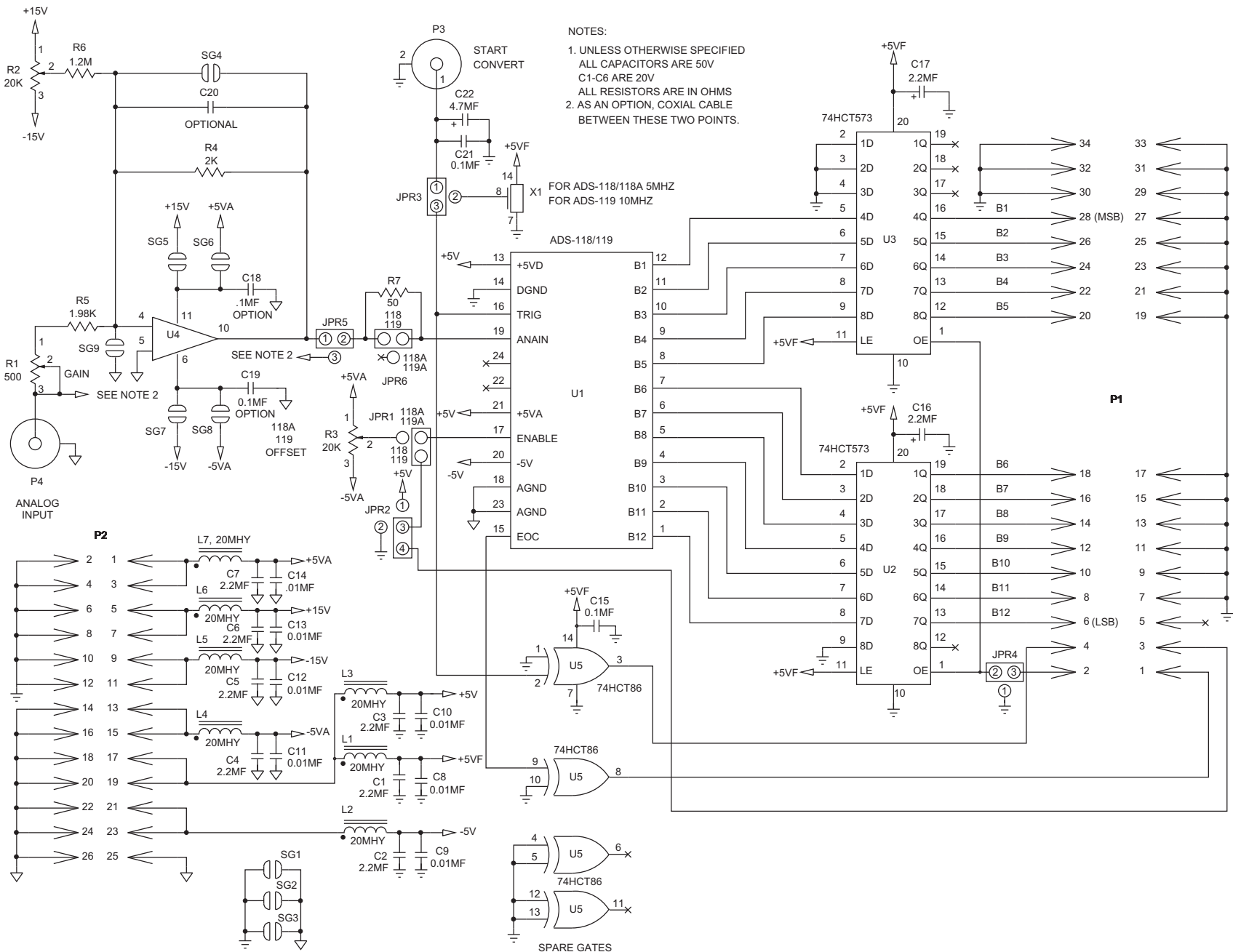
Figure 7. ADS-118/118A Evaluation Board Schematic (ADS-B118)
