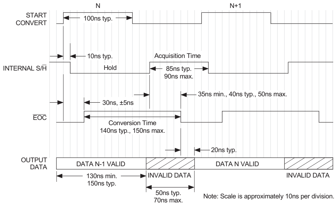
Figure 4. ADS-118/118A Timing Diagram
