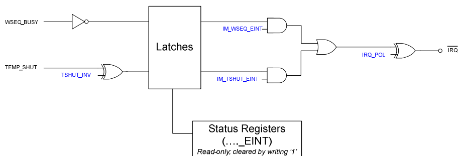
Figure 54 Interrupt Controller
