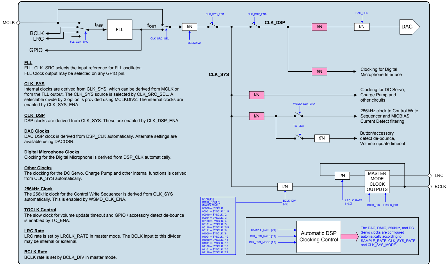
Figure 48 Clocking Overview
