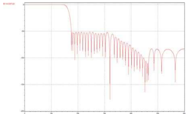
Figure 9 DAC Filter Response for CLK_SYS_MODE = 00b or 01b DAC_SB_FILT = 0b (Normal Filter) Sample Rate > 24\text{kHz}
