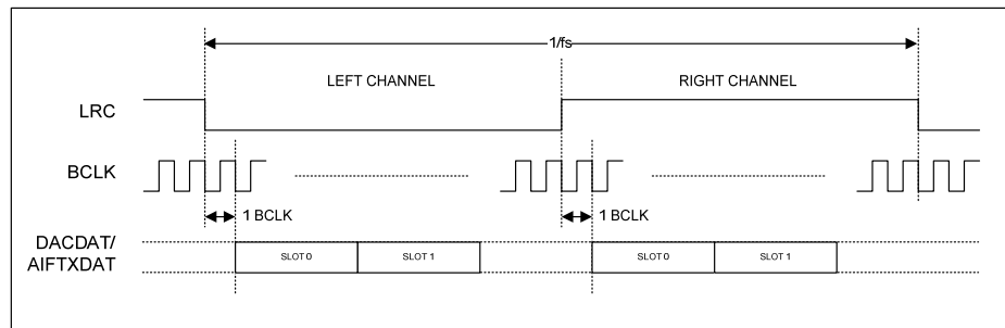
Figure 43 TDM in I²S Mode
