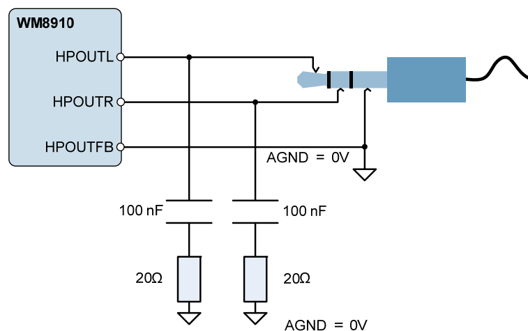
Figure 27 Zobel Network Components for HPOUTL, HPOUTR, LINEOUTL and LINEOUTR
