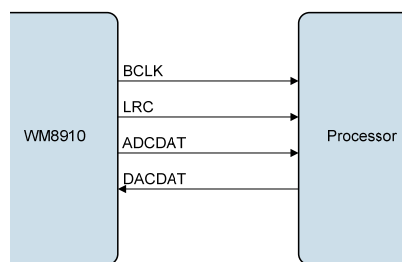
Figure 29 Master Mode
