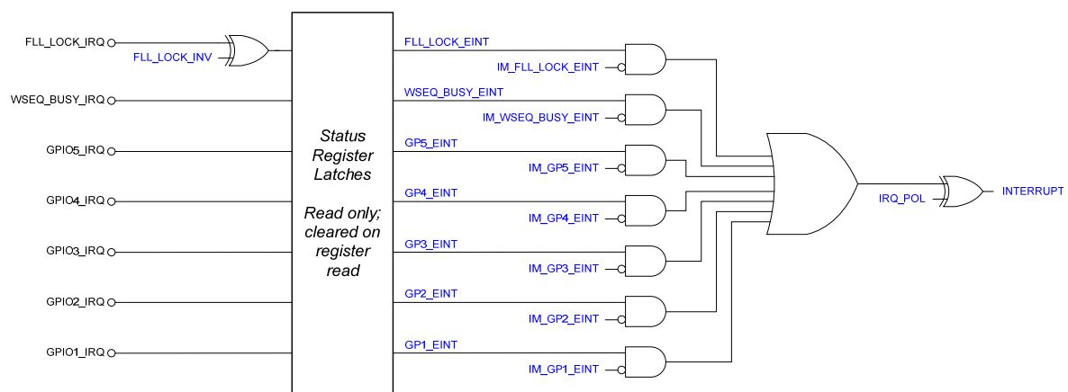
Figure 49 Interrupt Controller
