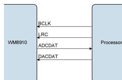
Figure 30 Slave Mode
