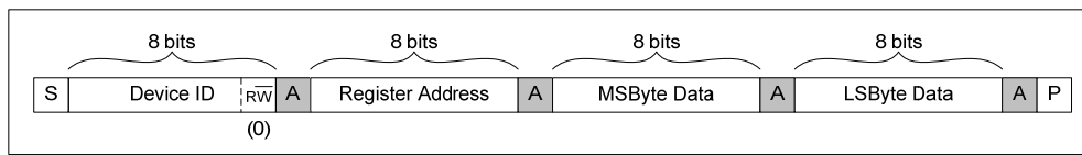
Figure 52 Single Register Write to Specified Address
