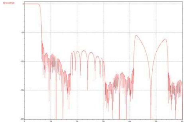
Figure 7 DAC Filter Response for CLK_SYS_MODE = 00b or 01b DAC_SB_FILT = 1b (Sloping StopBand Filter) Sample Rate \leq 24\text{kHz}
