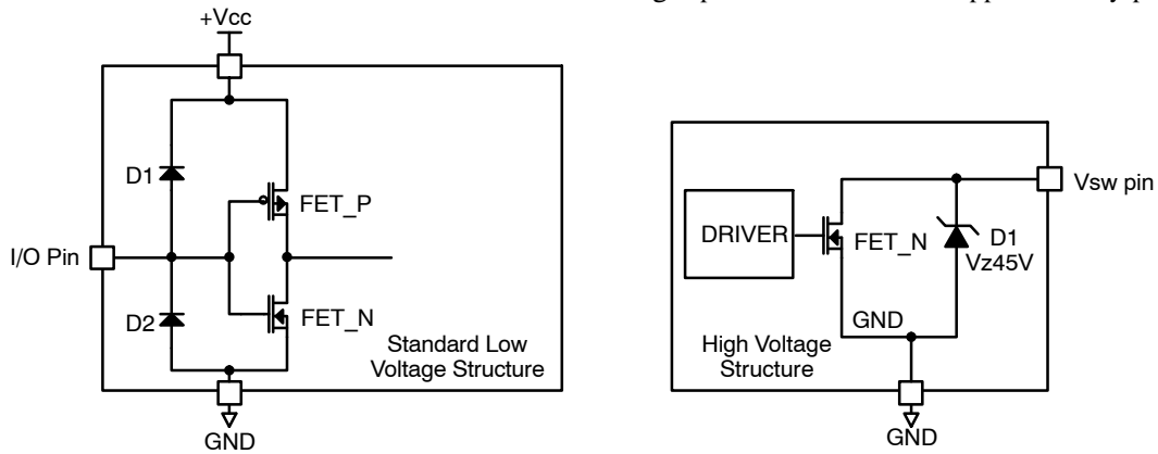
Figure 21. Typical ESD Protection Structures
