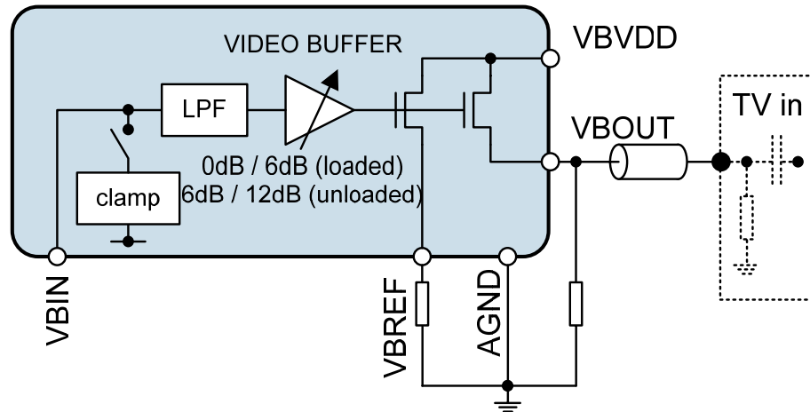
Figure 25 Video Buffer
