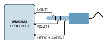
DC Coupled Headphone Output (OUT3SW = 00)
