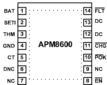
Figure 1 Pin Out
