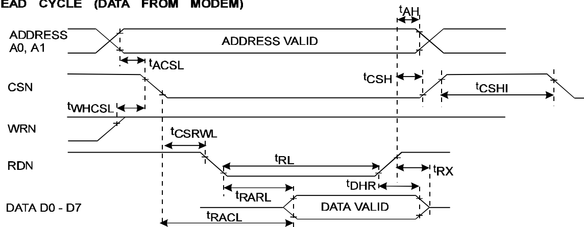
Figure 14 μC Parallel Interface Timings
